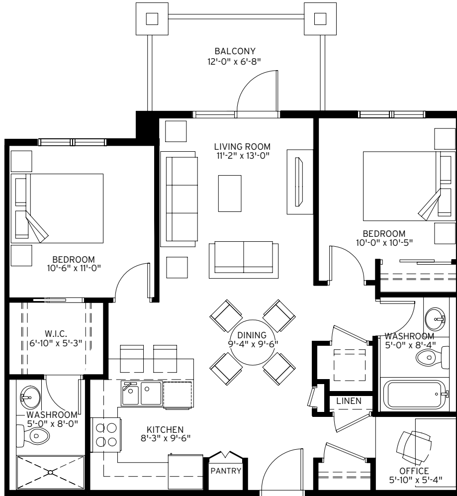
UNIT B1 ~ 898 SQ. FT. ~ TWO BEDROOM & DEN
