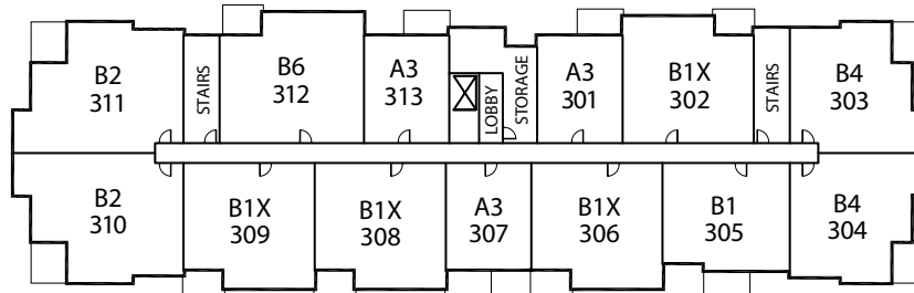
THIRD FLOOR
